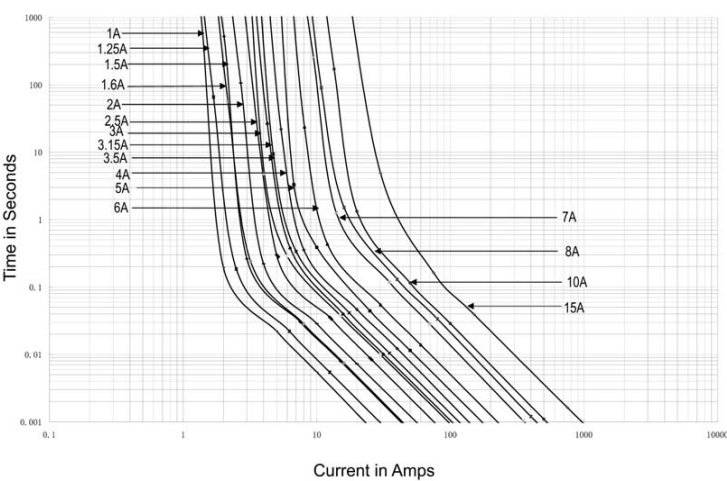
Time-Current Curve – GMA-R 1-15A
