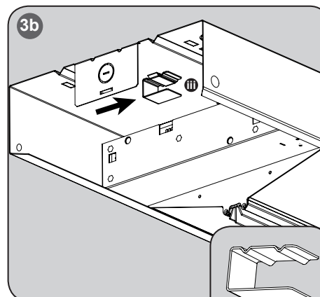
Stand-Off Bracket
