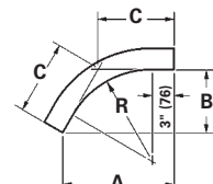
60° Vertical Outside
