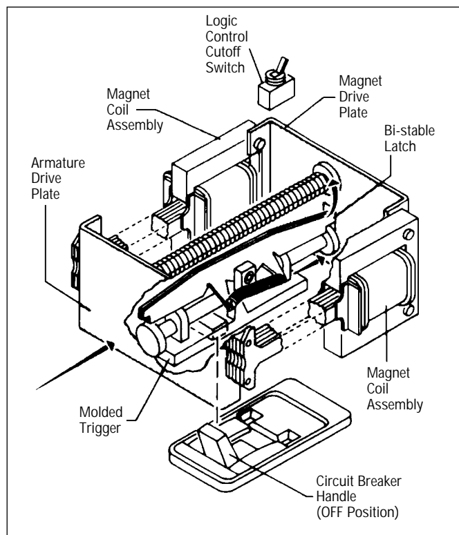
Figure 1-2 Circuit Breaker Handle in OPEN Position
