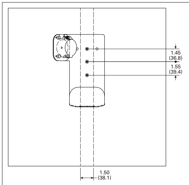
Figure 1. Mounting hole dimensions in inches (mm)
