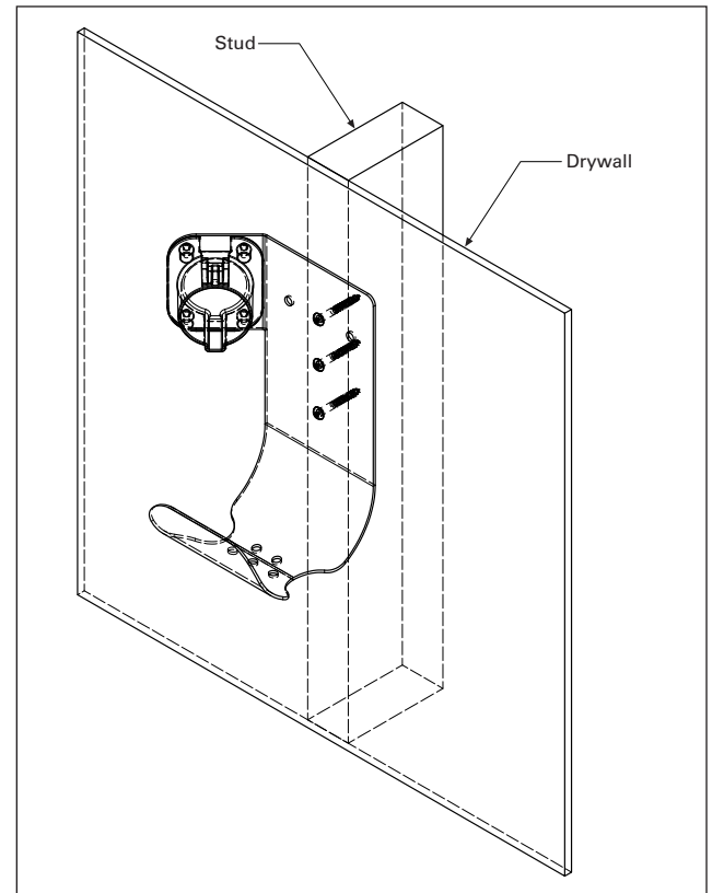
Figure 2. Attaching premium cord holster to wall
