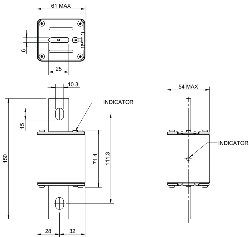
Dimensions (mm)- Size 2, bolted
