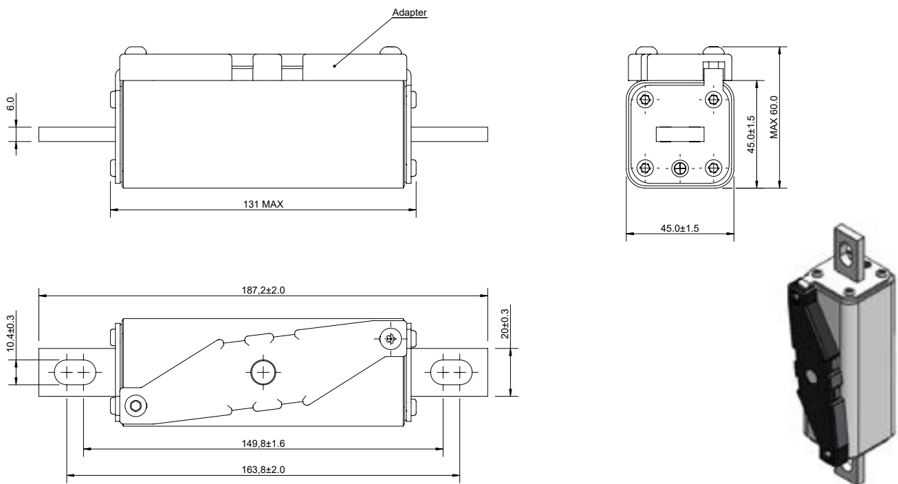
Dimensions (mm) - Size 01, bolted
