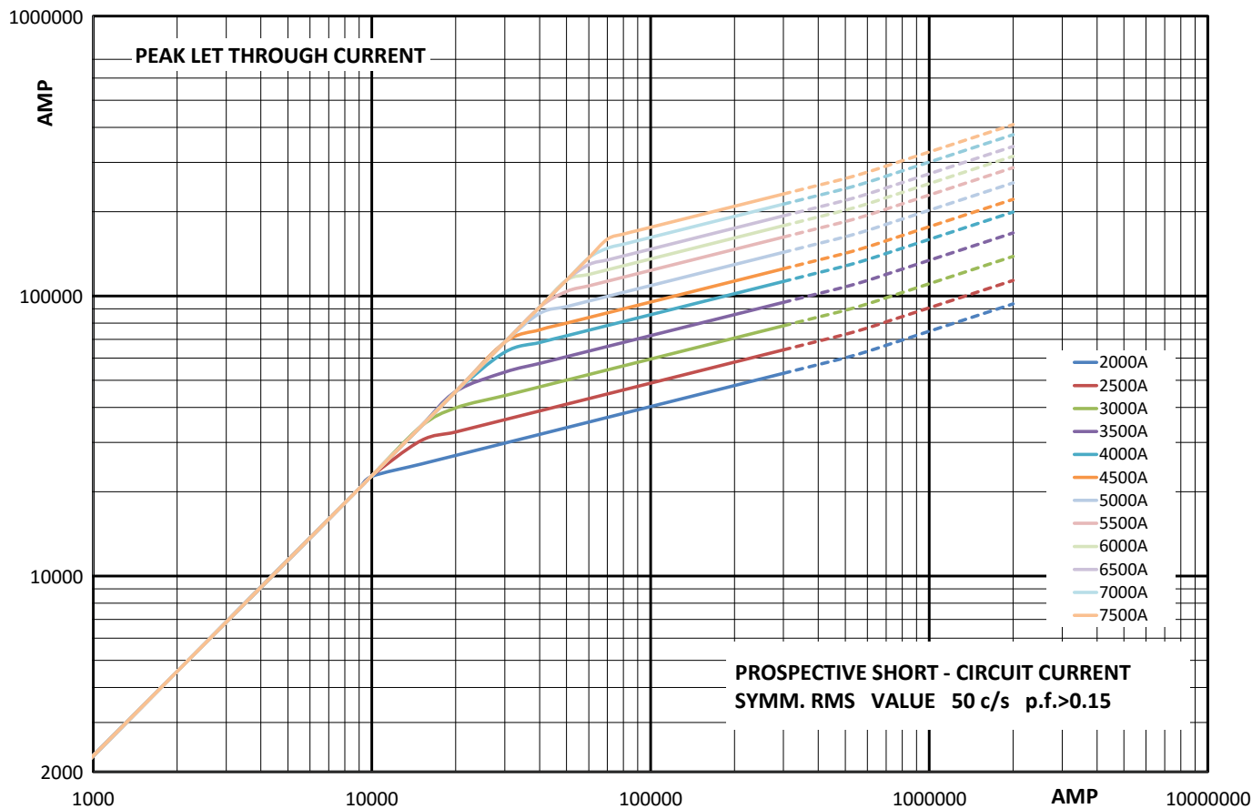
Cut-off curve - 2000 A to 7500 A
