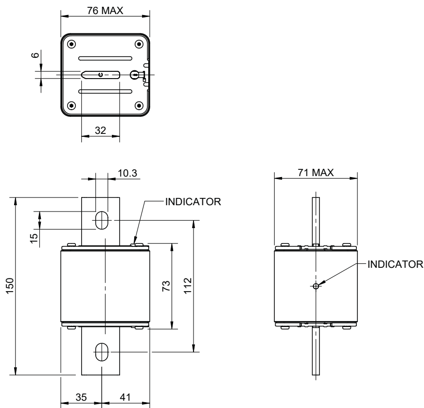
Dimensions (mm) - Size 3, bolted
