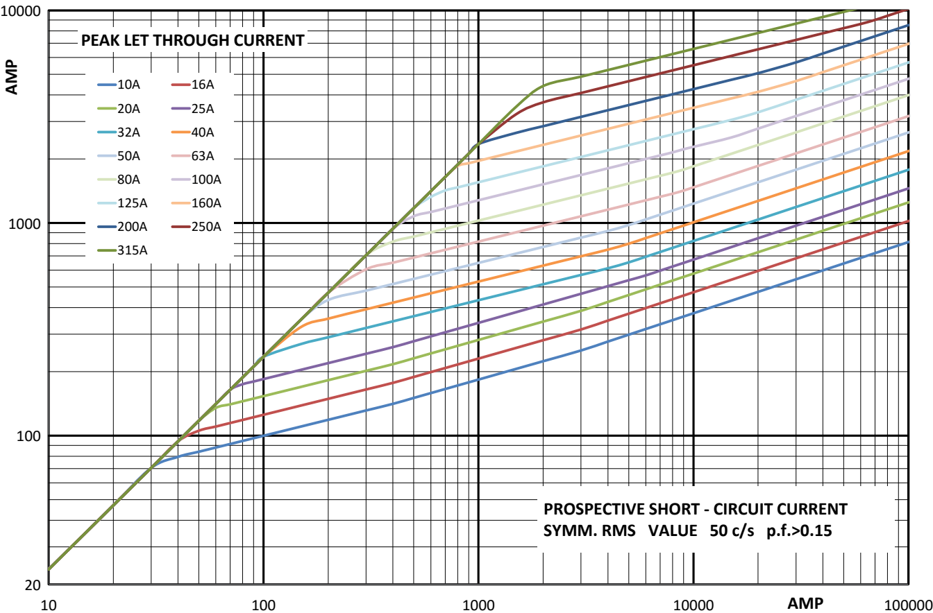
Cut-off curve - Size 000 - 10 A to 315 A
