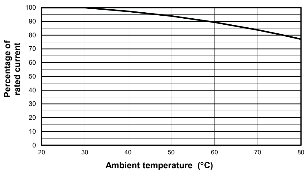
Temperature derating
