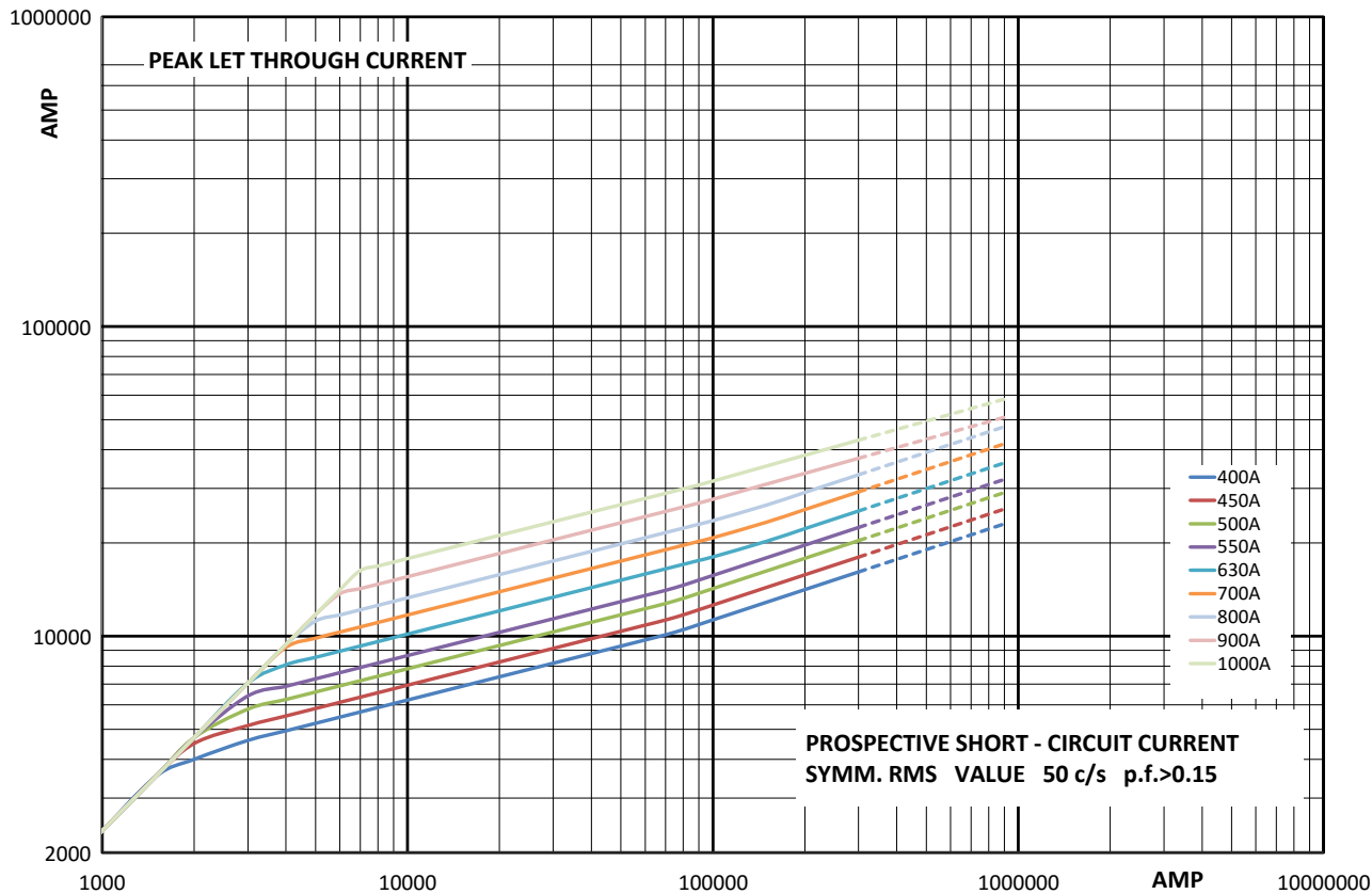
Cut-off curve - Size 2, 400 A to 1000 A
