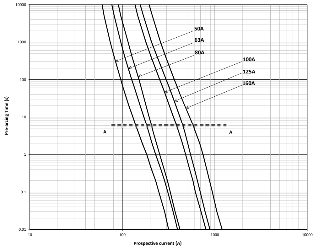
Time-current curve - 170M2000 to 170M2005, 50 A to 160 A
