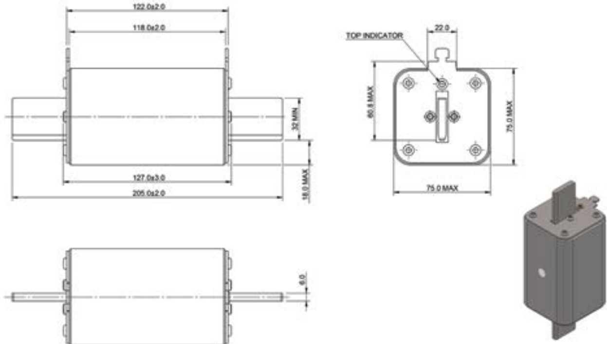
Dimensions (mm) - Size 3, bladed
