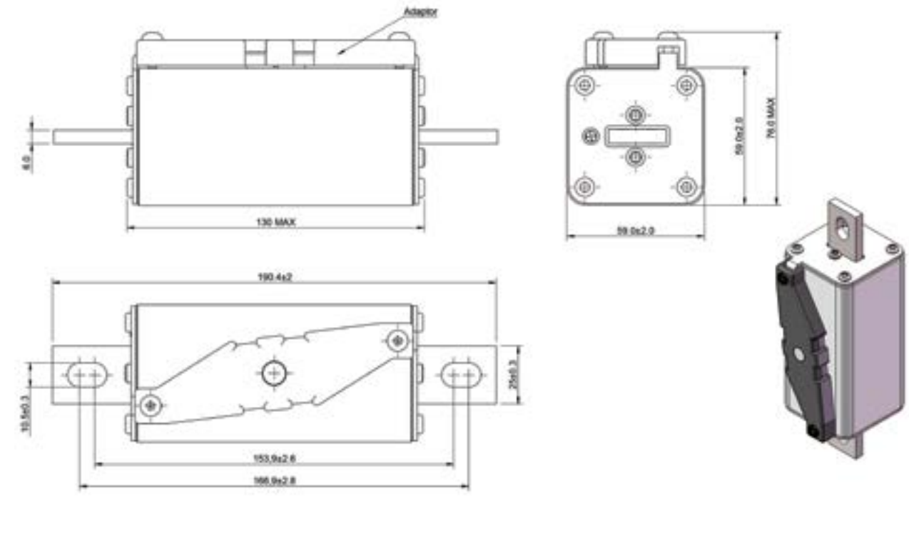
Dimensions (mm) - Size 2, bolted
