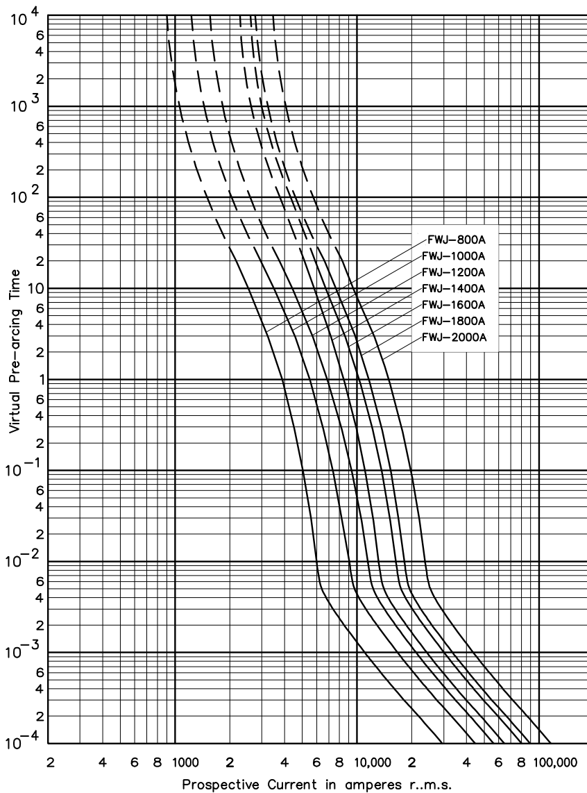
Time-current curve - 800 A to 2000 A
