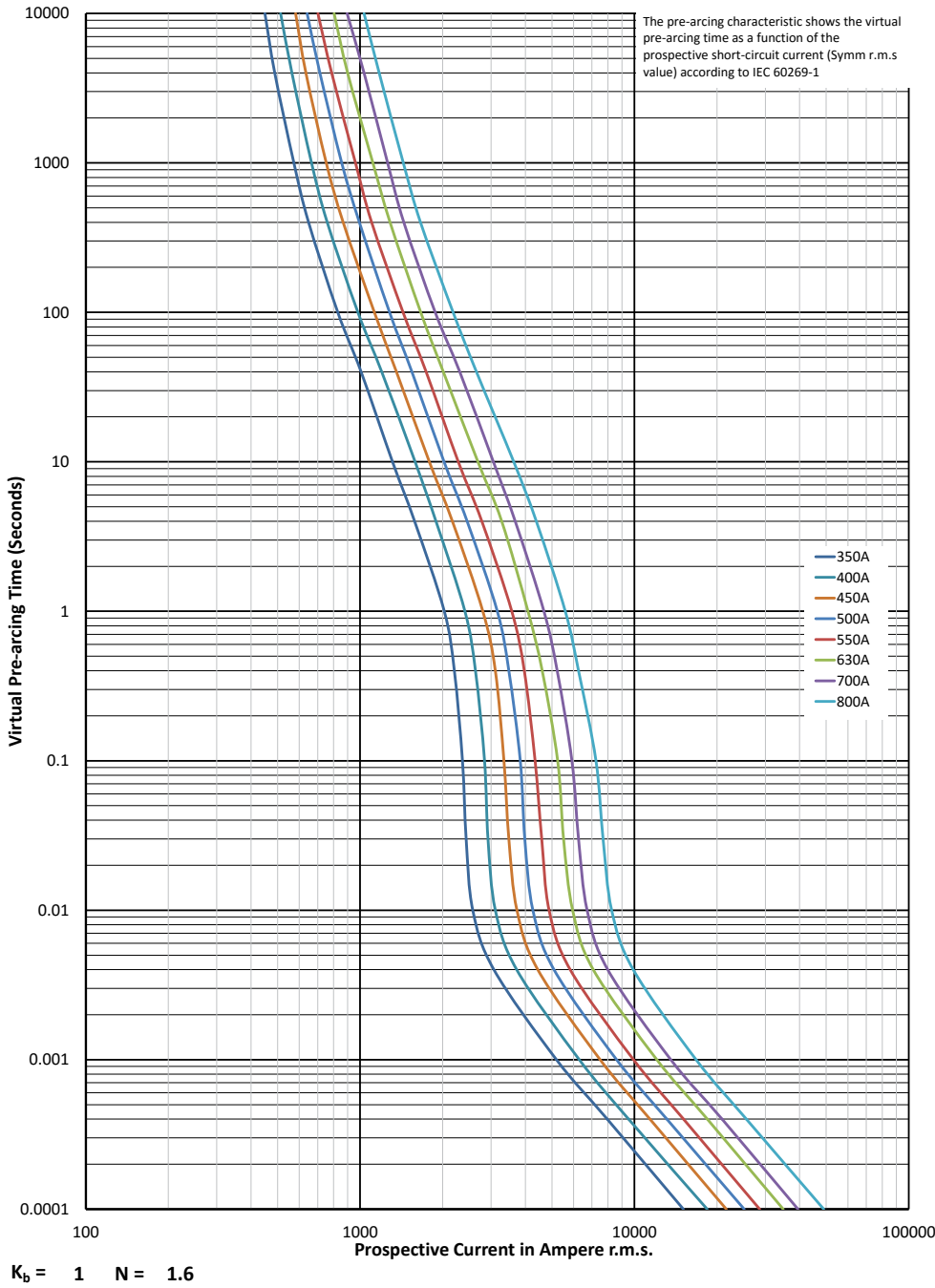
Time-current curve - Size 3, 350 A to 800 A
