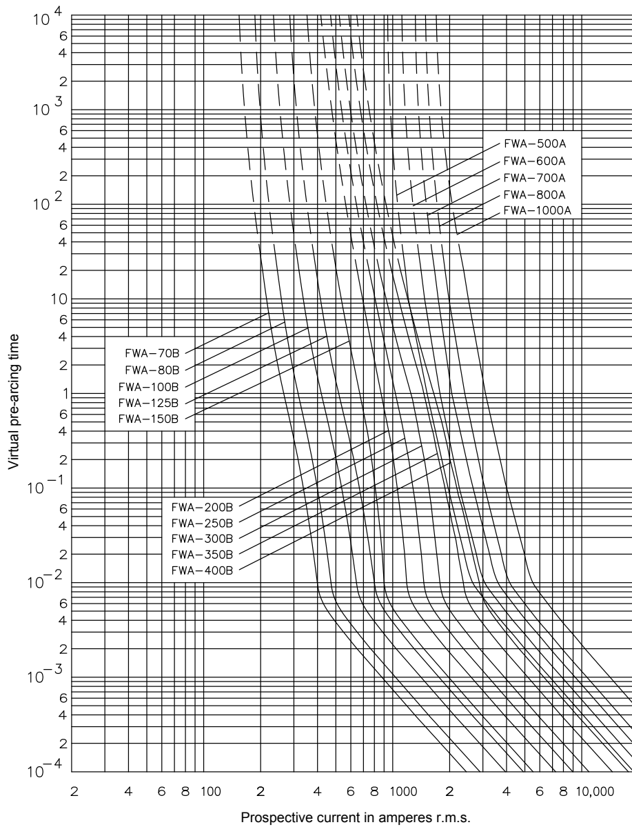
Time-current curve - 70 A to 1000 A
