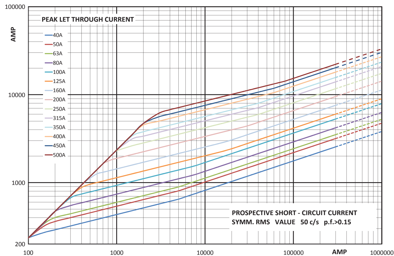
Cut-off curve - Size 1*, 40 A to 500 A
