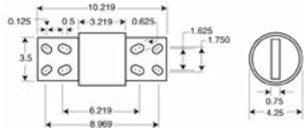
Dimensions (in) - 1400 A and 1600 A
