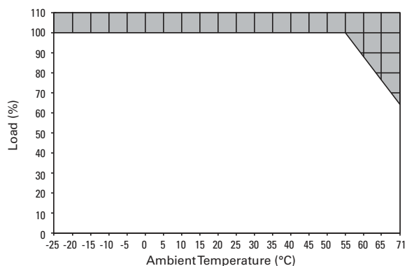
Vertical Mounting Position PSL30E24RP
