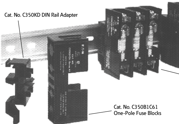
Cat. No. C350BD3C61 Three-Pole with Adapter (Mounted on DIN Rail)
