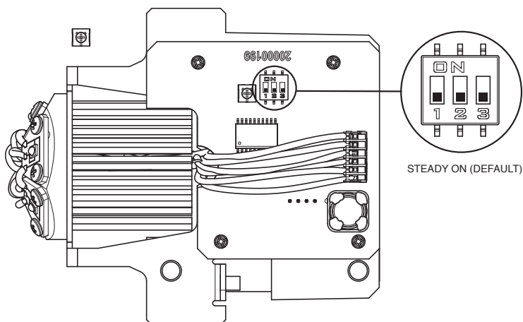
Figure 9 Location of DIP switch for flash patterns
