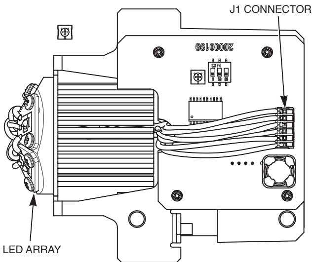
Figure 11 LED array and connector
