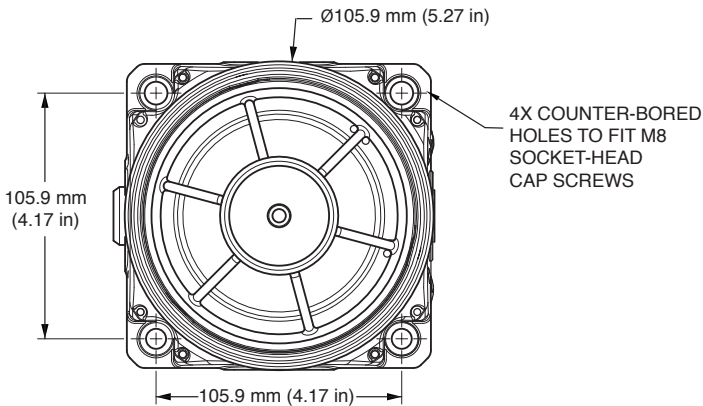
Figure 2 Front view of Ex d beacon
