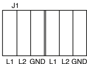
Figure 7 IN/OUT PCB connections for Ex d 120-240 Vac
