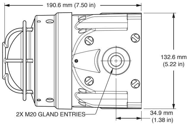
Figure 3 Side view of Ex d beacon
