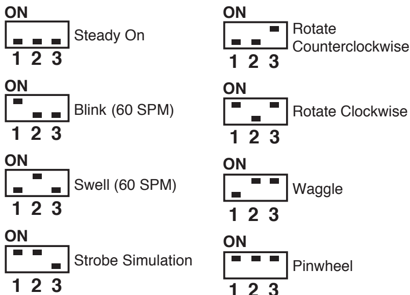
Figure 10 Switch settings for flash patterns
