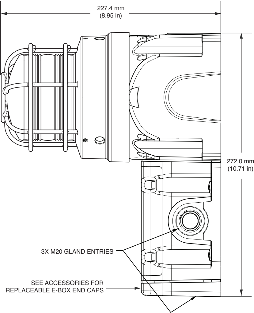
Figure 5 Side view of Ex de surface mount
