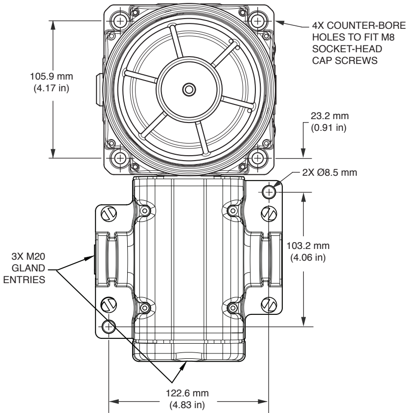
Figure 4 Front view of Ex de surface mount
