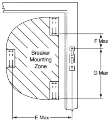
Circuit Breaker Mounting Zone Dimensions
