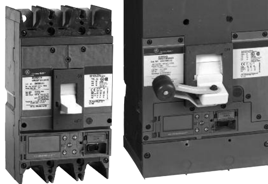
Spectra™ SG600 and SK1200 Breakers with microEntelliGuard™ Trip Units
