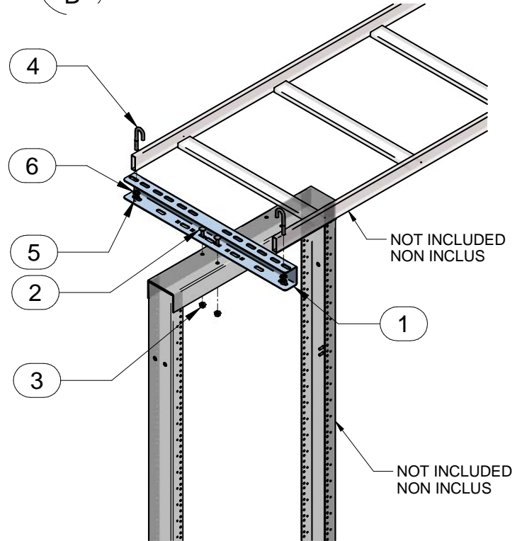
ITEM 6 LOCK WASHER, 3/16 QTY 2
