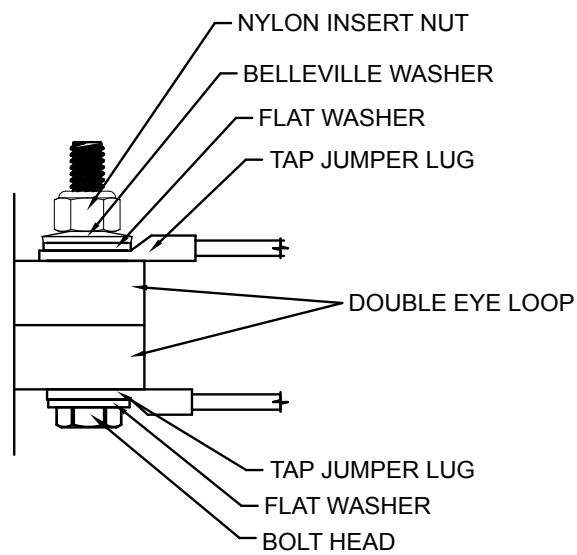
Double Conductor Eyeloop Tap Lugs
