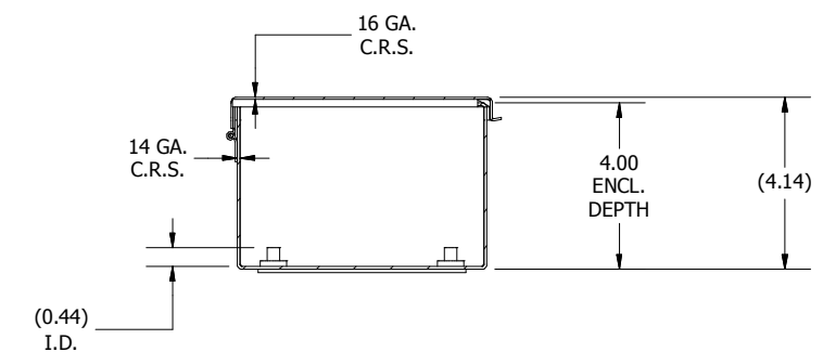
SECTION L-L VIEW (INSIDE TOP OF ENCL.)
