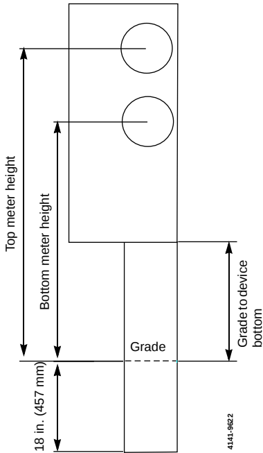
Figure 1: METER-PAK Device Dimensions
