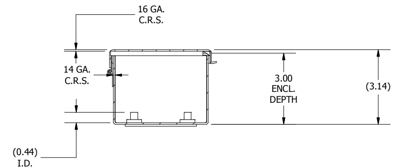
SECTION L-L VIEW (INSIDE TOP OF ENCL.)
