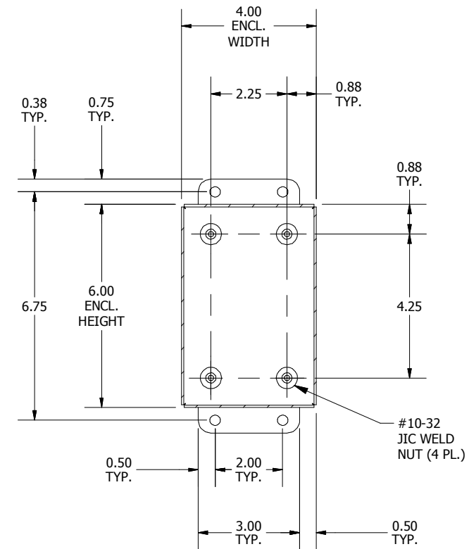
SECTION K-K (INSIDE BACK OF ENCLOSURE)
