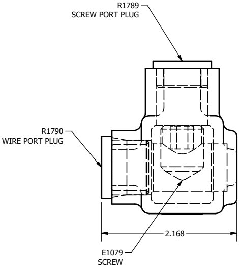
VIEW A-A SCALE 1.5:1
