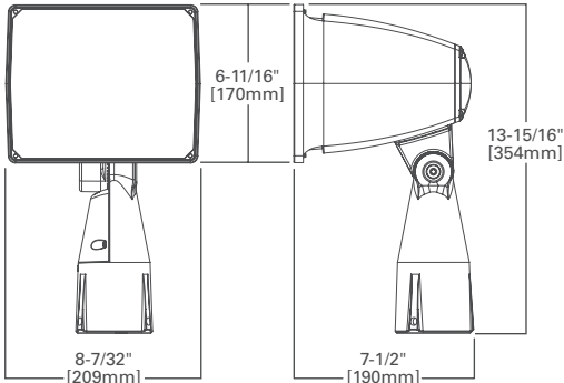
Slipfitter mount
