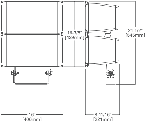
Trunnion mount
