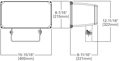
Trunnion mount
