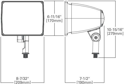
Knuckle mount
