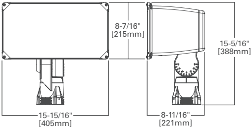
Slipfitter mount
