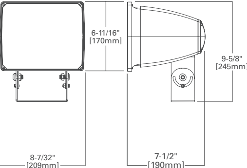
Yoke mount
