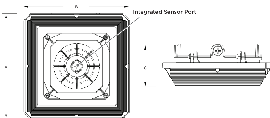
Microwave Sensor (86-218)
