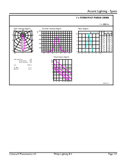
Accent Lighting Spots - 36PAR38/PER/830/F25/ND/120V 6/1FB
