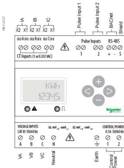
EM3500 parts and connection terminals
