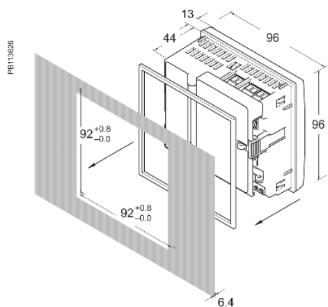
Dimensions PM5350IB
