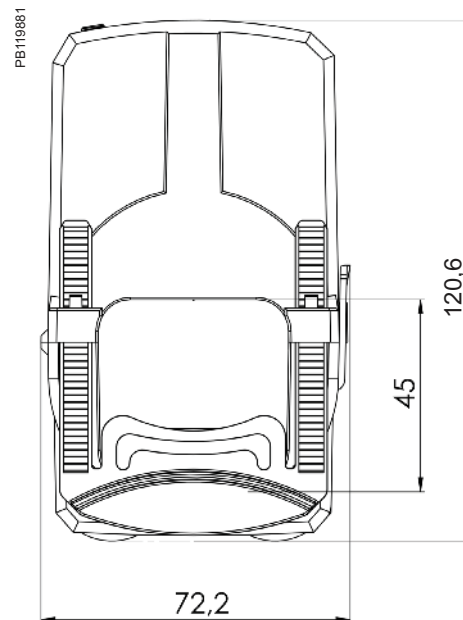
HP Dimensions
