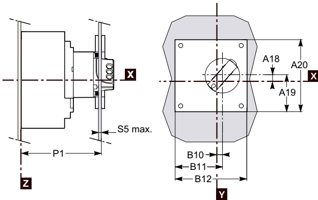
Operating Handle
