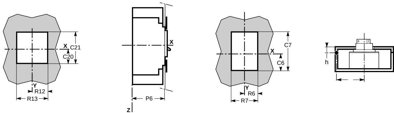
With Toggle Boot
