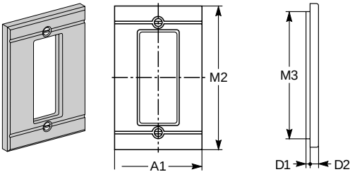
For Toggle
