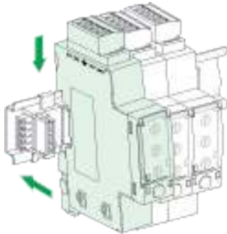
Up to Twelve Stacked IFMs
