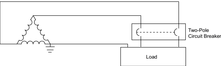
Three-Phase 240 Vac Corner-Grounded Delta System
