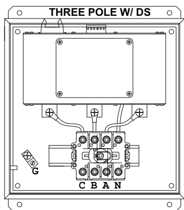
Figure 6: Three-Phase, Three- or Four-Wire, High-Leg Delta Installation with Integral Switch
