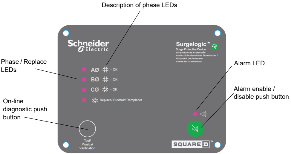
Figure 8: Three-Phase Diagnostic Display Panel
