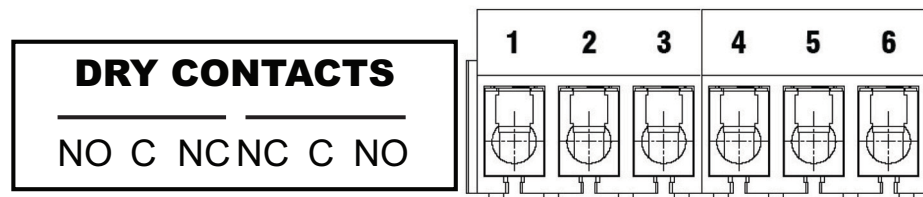
Figure 10: Dry Contact Configuration
