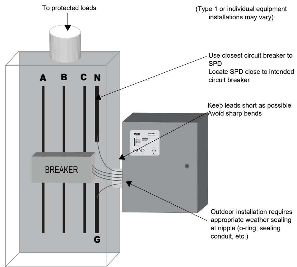
Figure 3: Typical Panel Installation
