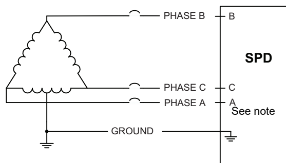
Figure 6: Three-Phase, Three- or Four-Wire, High-Leg Delta Installation with Integral Switch
