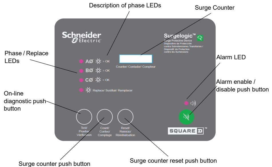
Figure 9: Three-Phase Diagnostic Display Panel with Surge Counter
