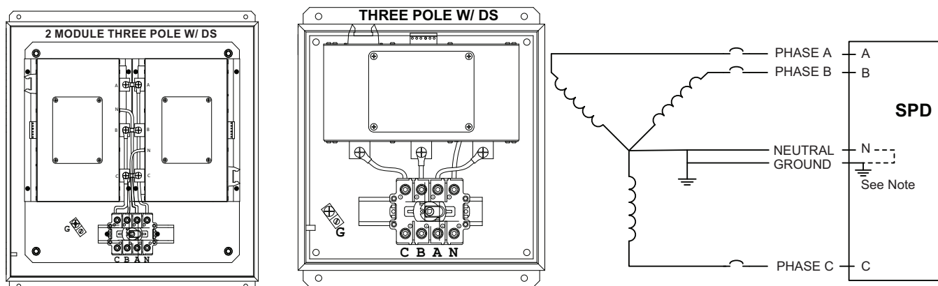
Figure 5: Three-Phase, Three- or Four-Wire, Grounded Wye Installation with Integral Switch
