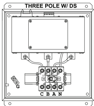
Figure 7: Three-Phase, Three-Wire + Ground, Delta Installation
