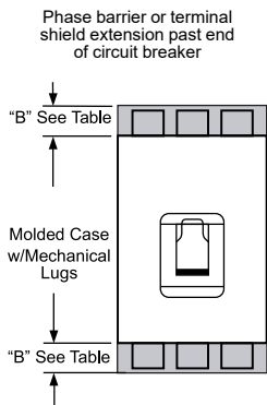
H-Frame Short Lug Shield
