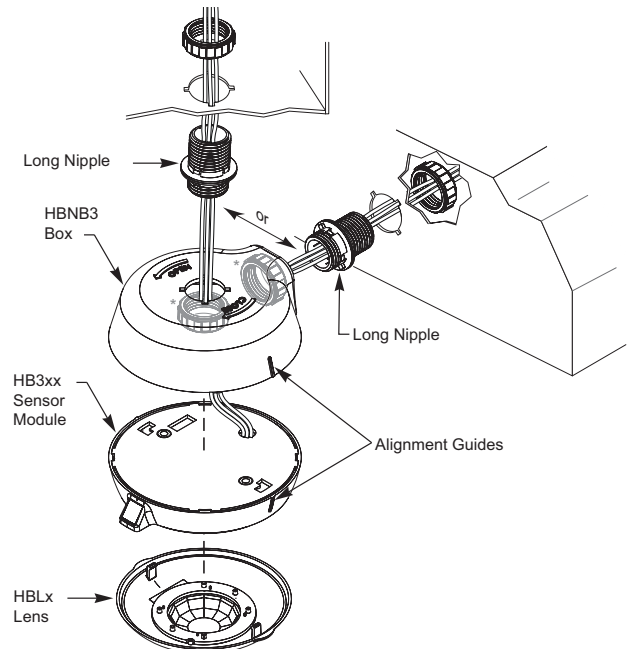
Fig. 3: Mounting to Fixture with HBNB3
