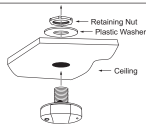
Figure 3: Ceiling tile mount
