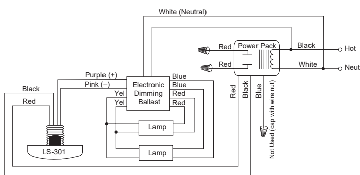
Typical Wiring
