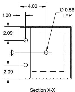
Section X-X
