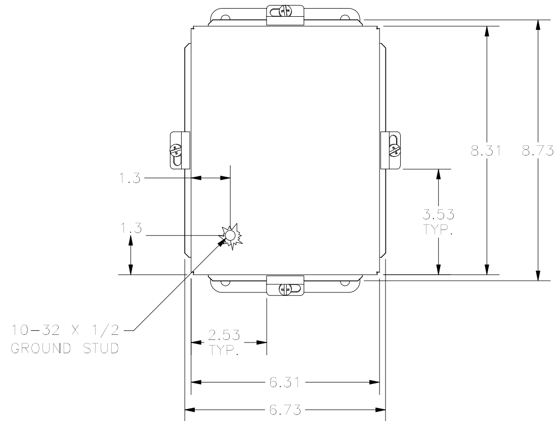
FRONT VIEW
