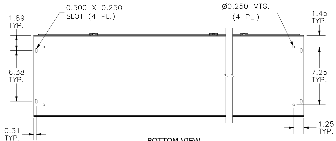
BOTTOM VIEW
