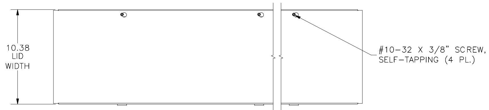
TOP VIEW
