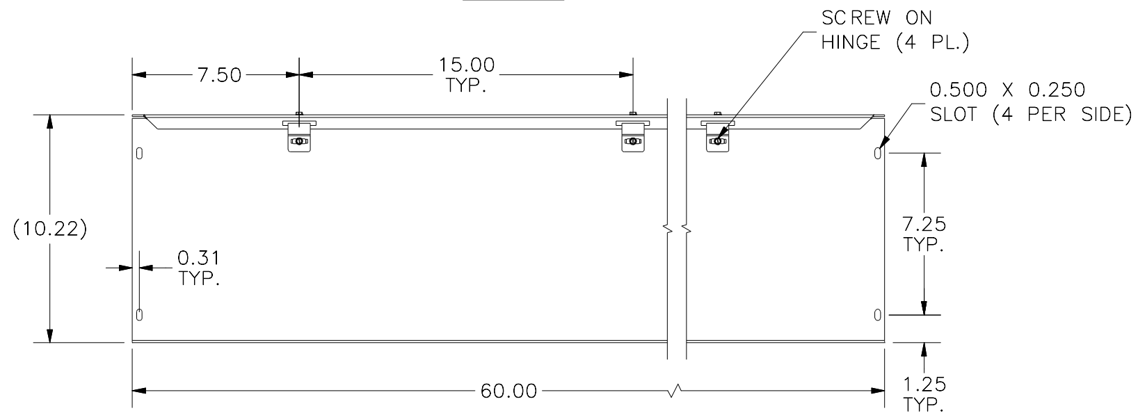
FRONT VIEW
