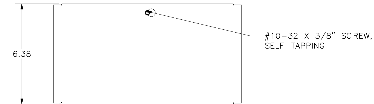
TOP VIEW
