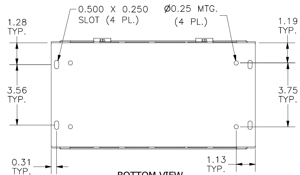
BOTTOM VIEW
