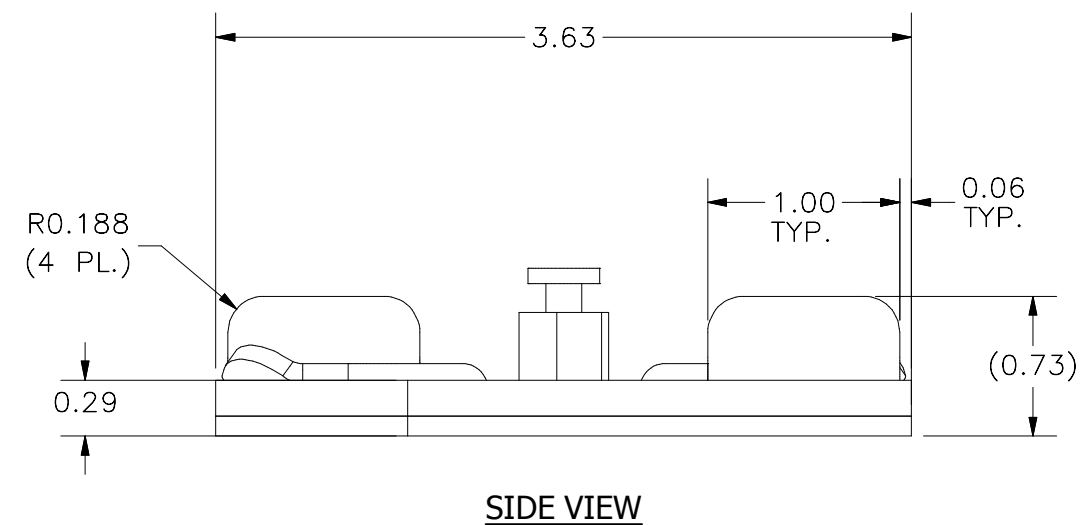
NUT REMOVED
