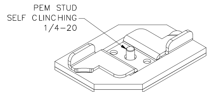
NUT REMOVED
