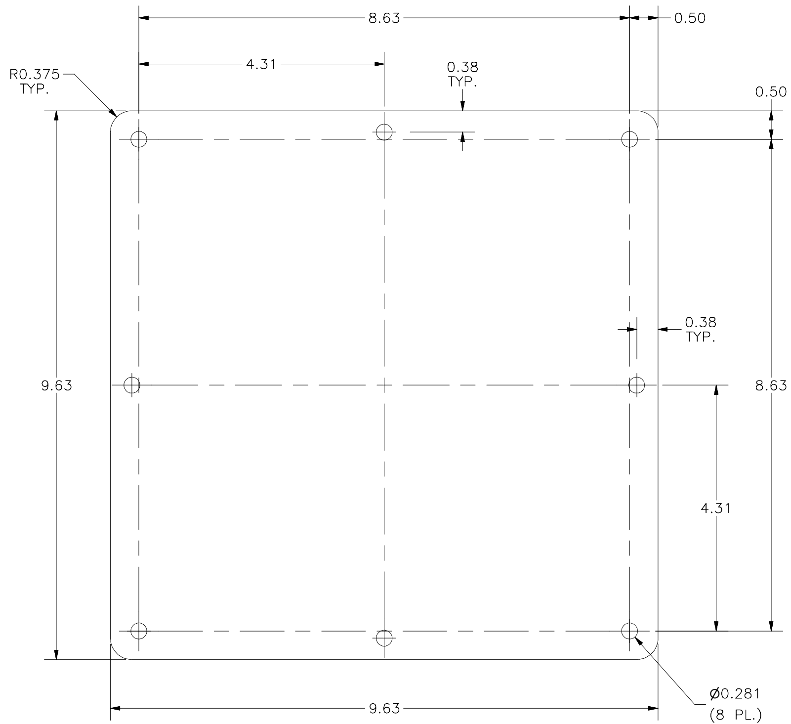
FRONT VIEW
