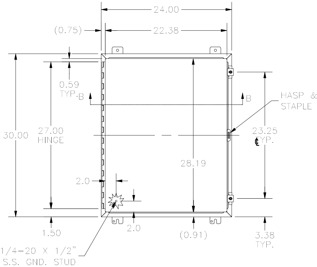
FRONT VIEW
