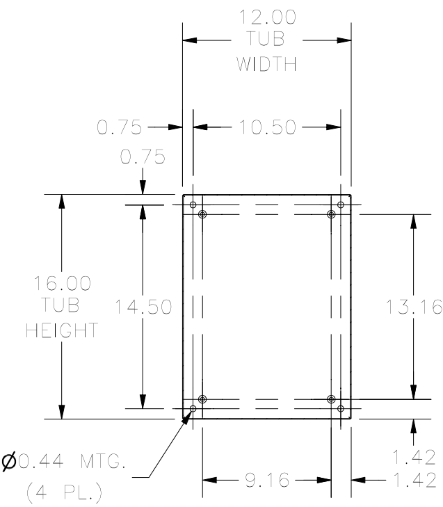
SECTION Y-Y (INSIDE BACK OF ENCLOSURE)
