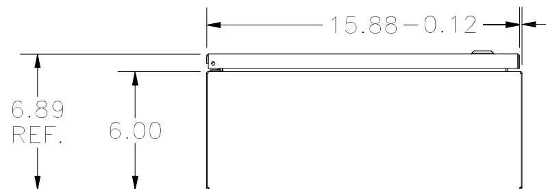
BOTTOM VIEW
