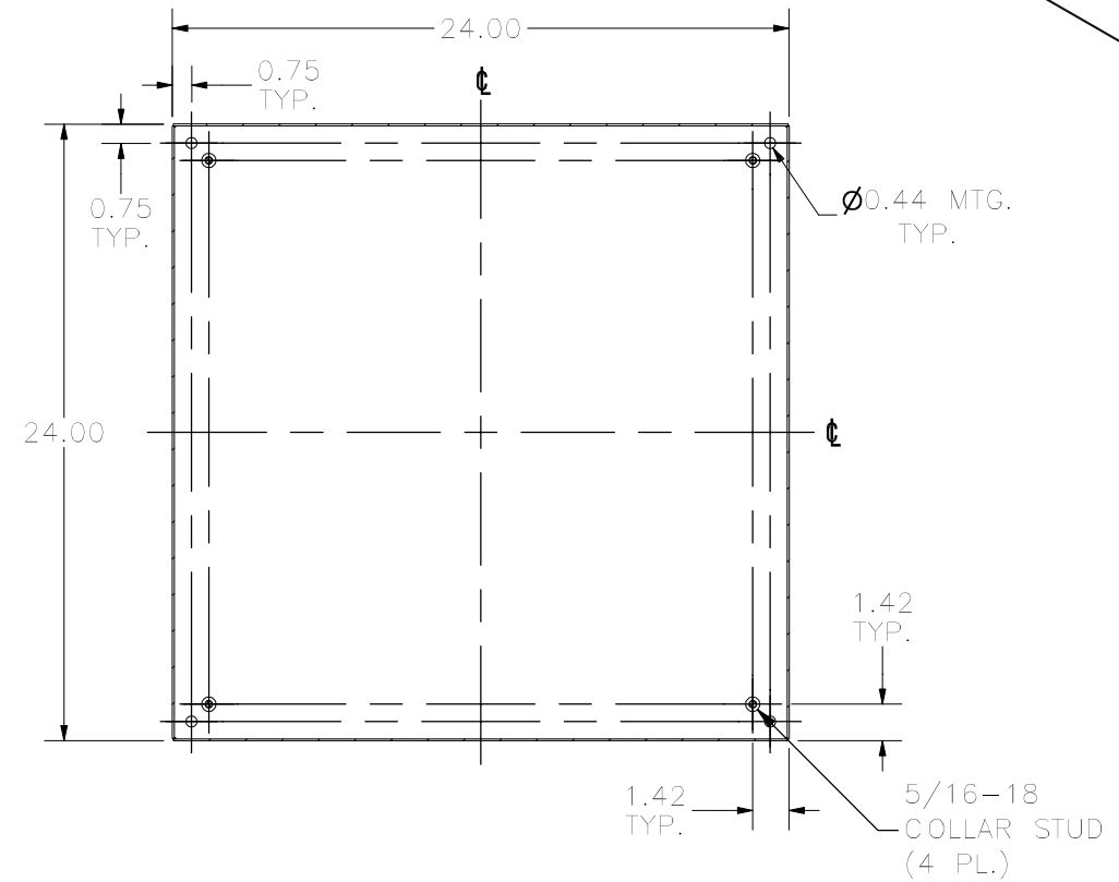
SECTION D-D VIEW (INSIDE BACK OF ENCLOSURE)
