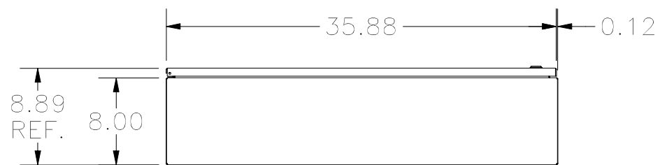
BOTTOM VIEW
