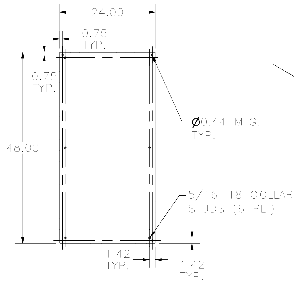
SECTION A-A (INSIDE BACK OF ENCLOSURE)
