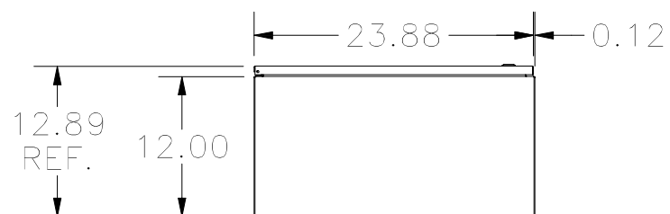
BOTTOM VIEW
