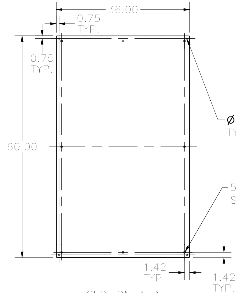
SECTION A-A (INSIDE BACK OF ENCLOSURE)
