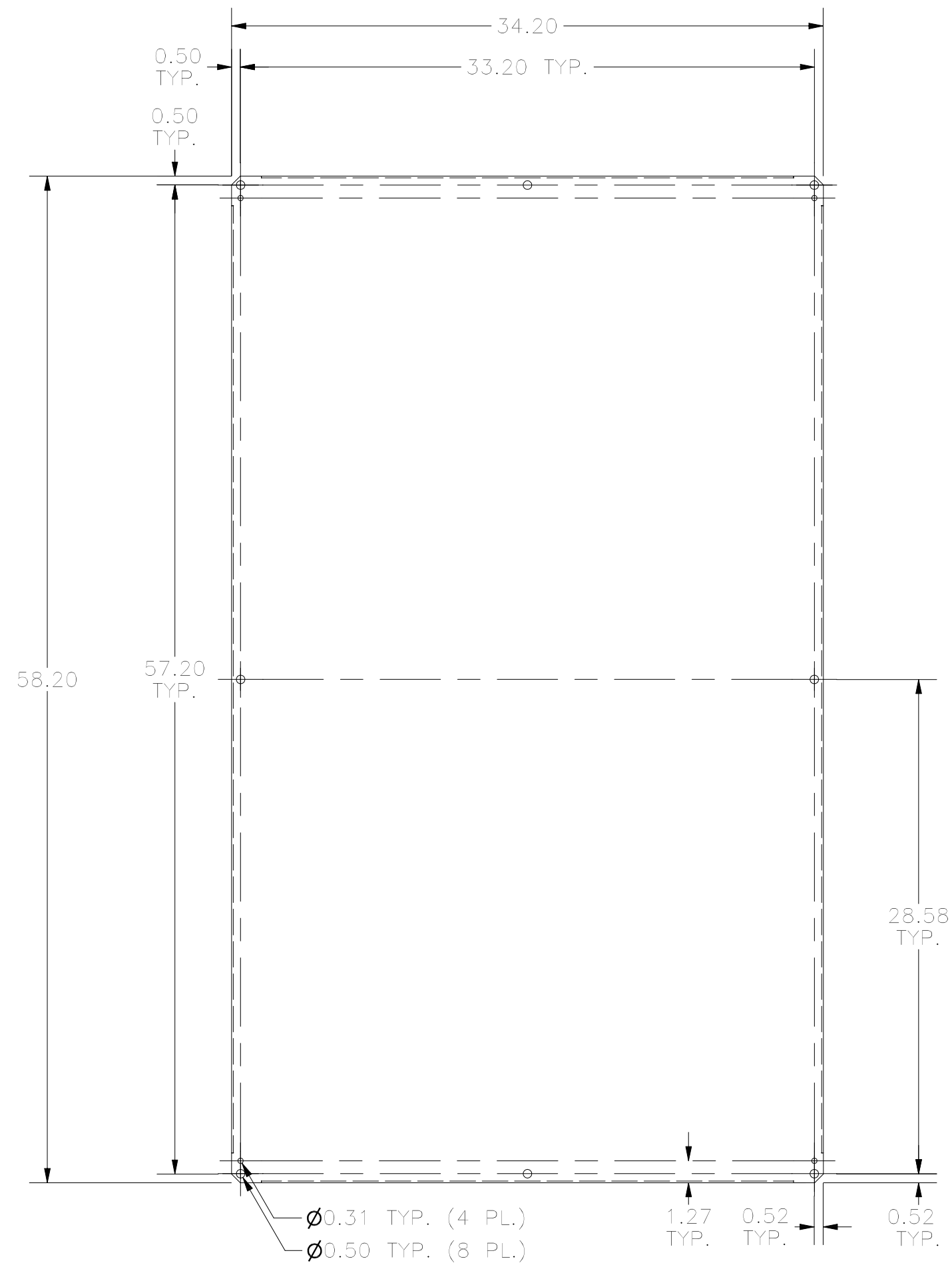
FRONT VIEW
