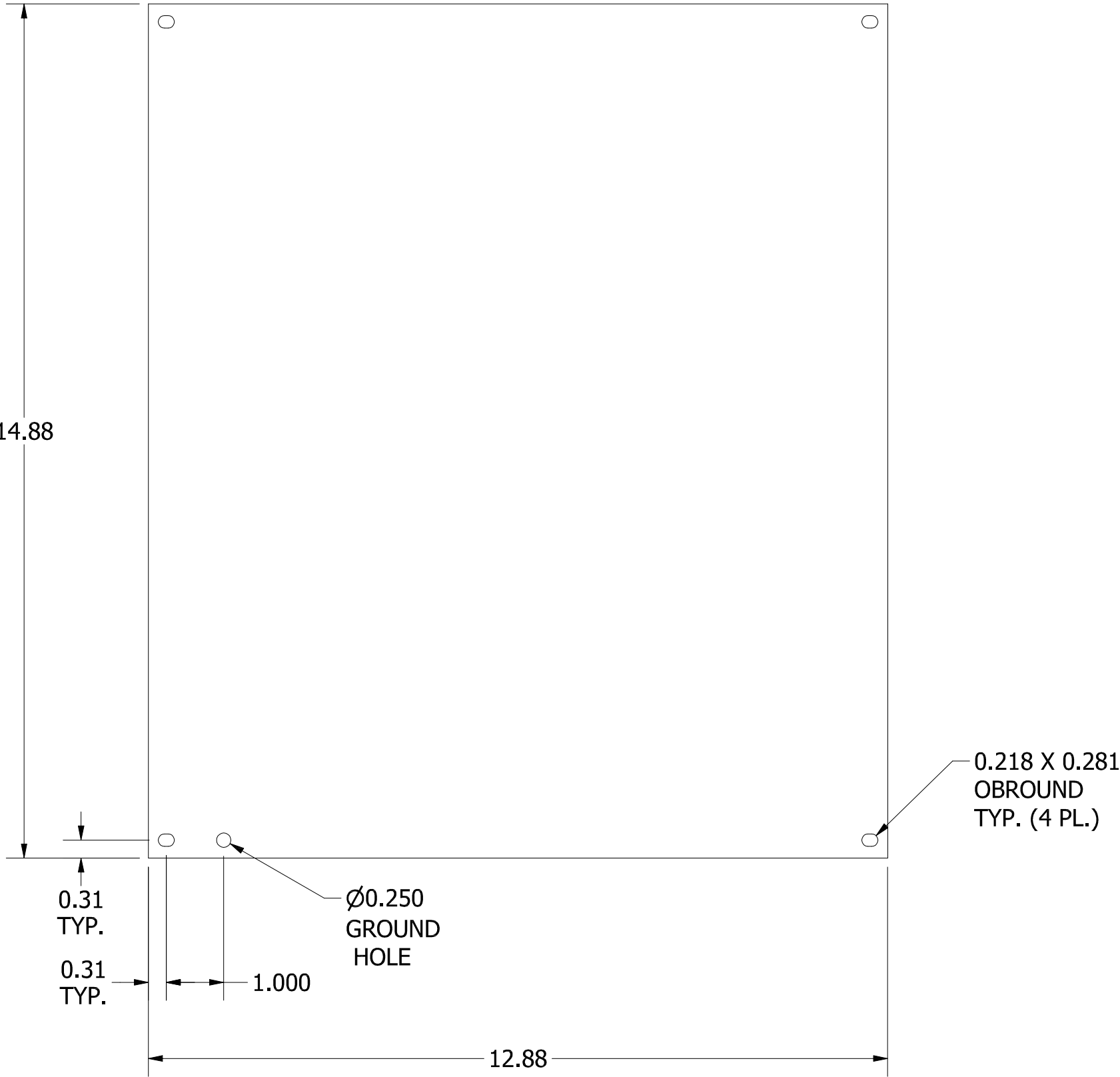
FRONT VIEW
