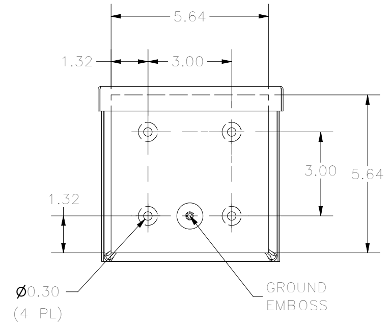
BACK VIEW
