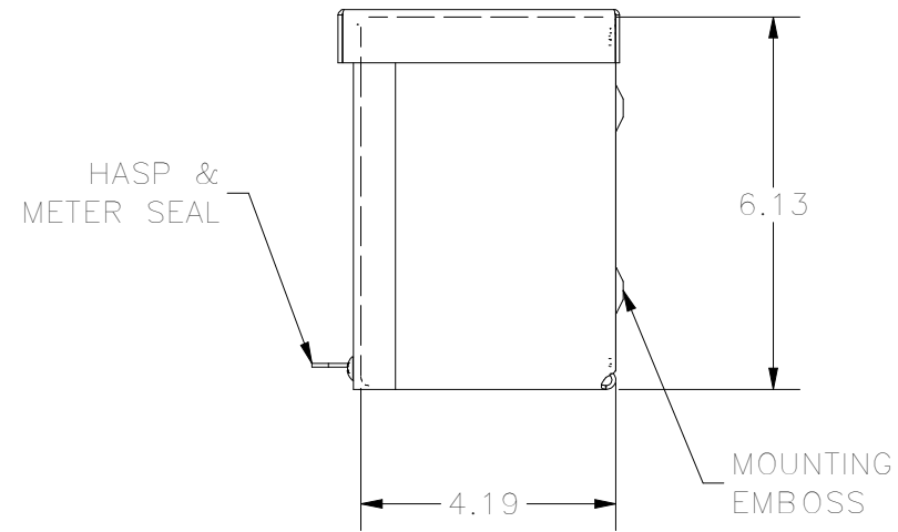
RIGHT VIEW
