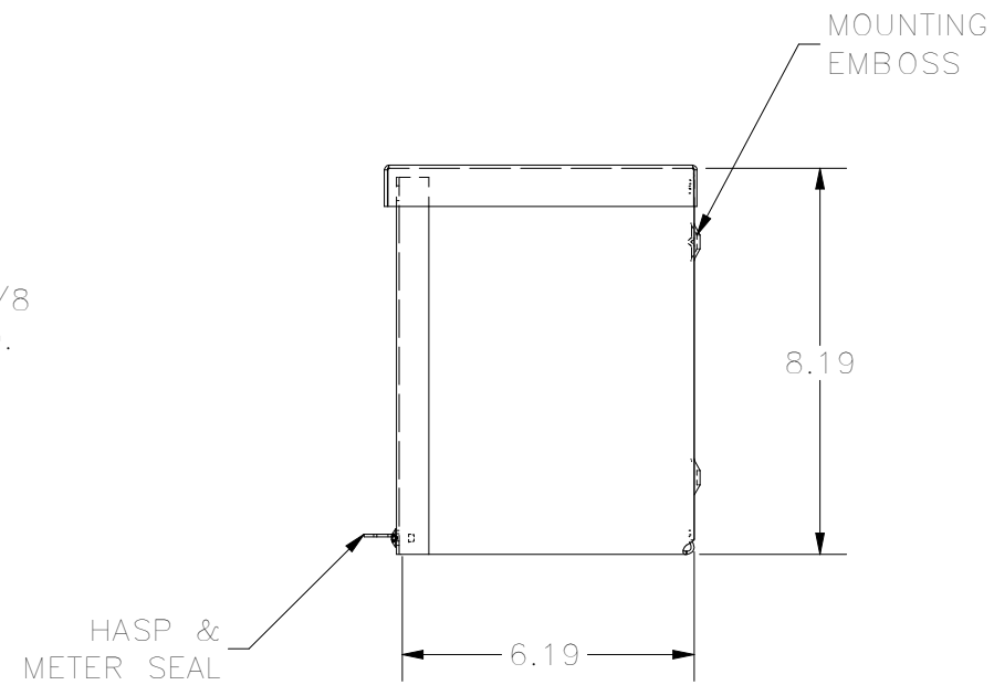
RIGHT VIEW
