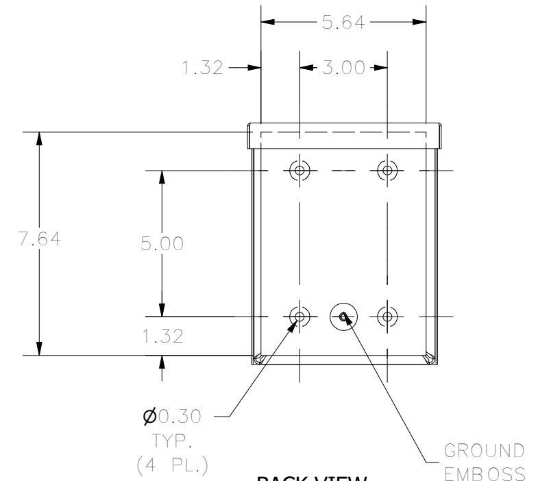
BACK VIEW
