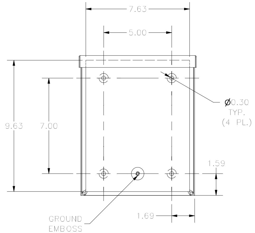
BACK VIEW
