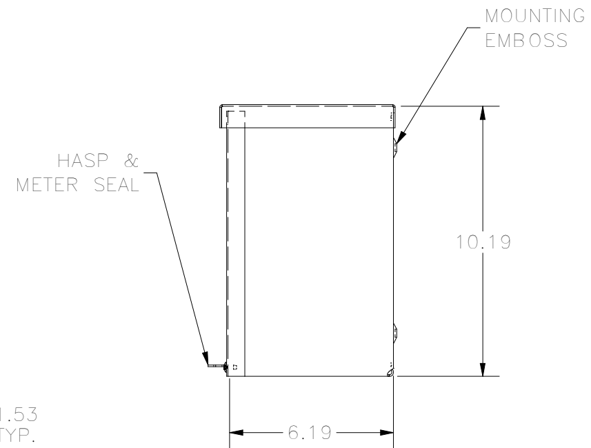
RIGHT VIEW
