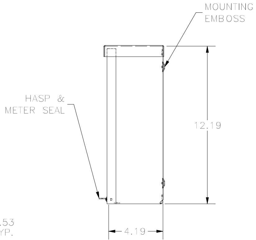
RIGHT VIEW
