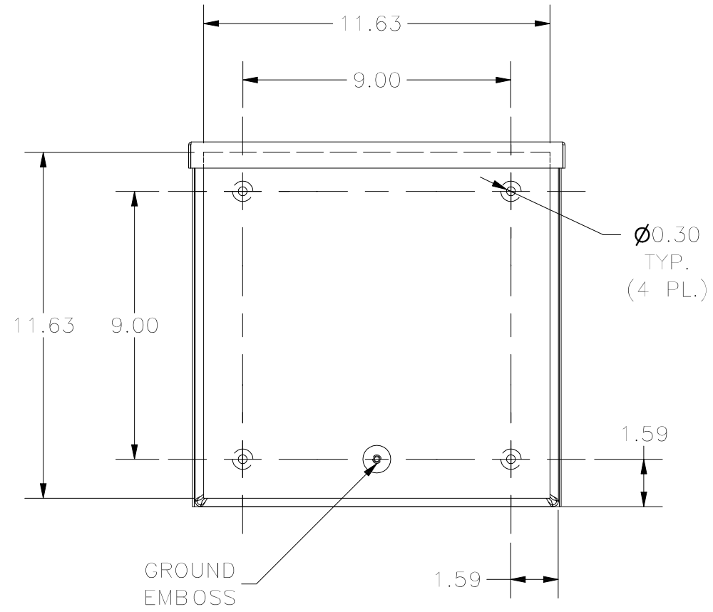
BACK VIEW
