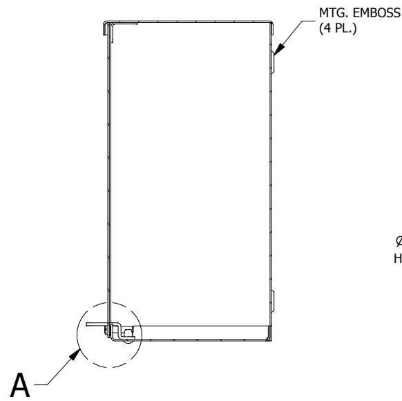
SECTION A-A (INSIDE LEFT OF ENCL.)
