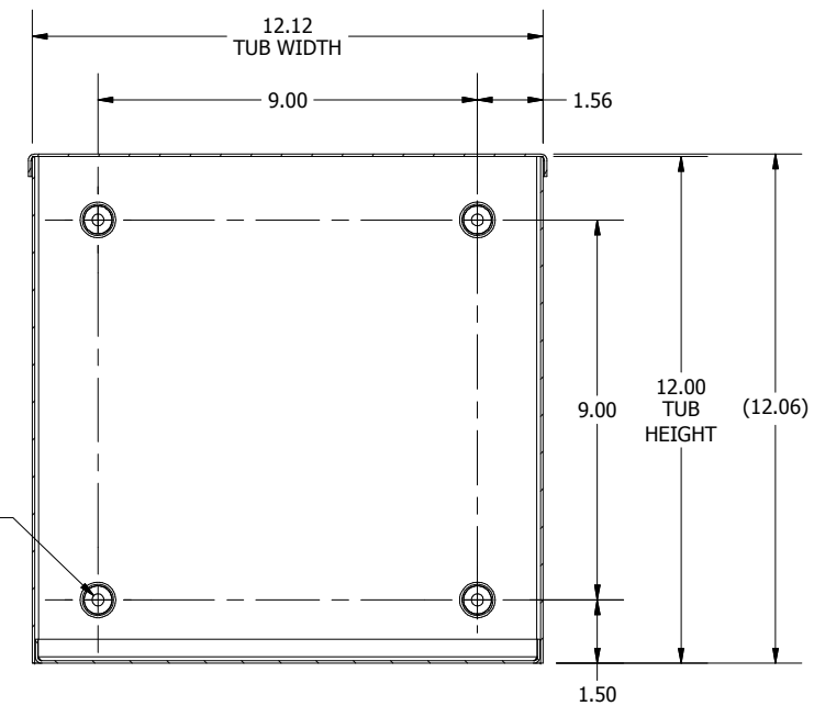
SECTION B-B (INSIDE BACK OF ENCL.)
