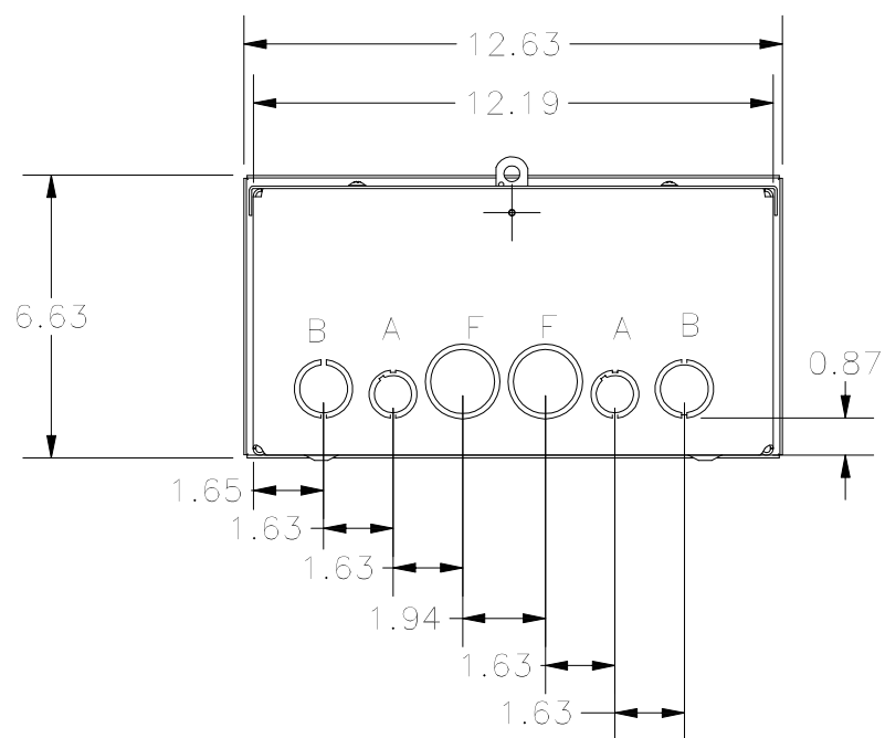
BOTTOM VIEW
