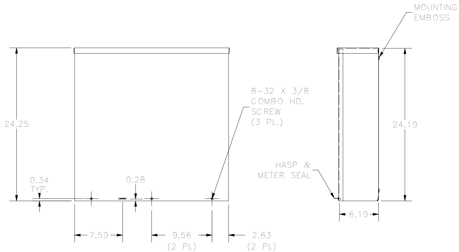
FRONT VIEW
