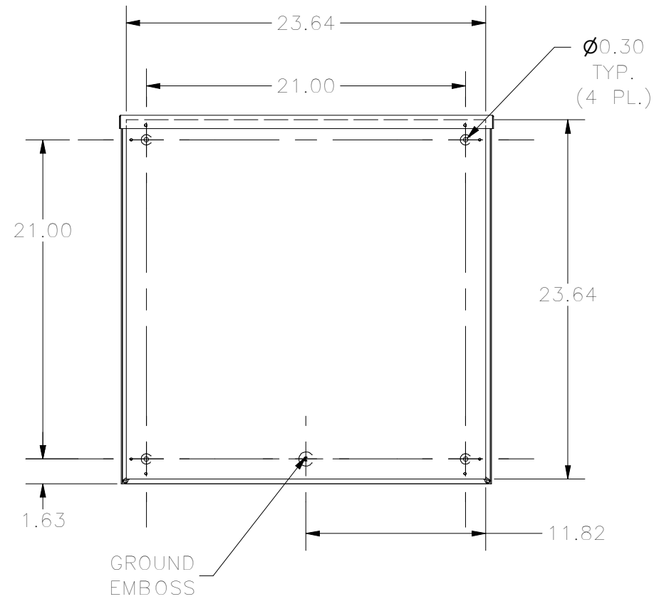
BACK VIEW
