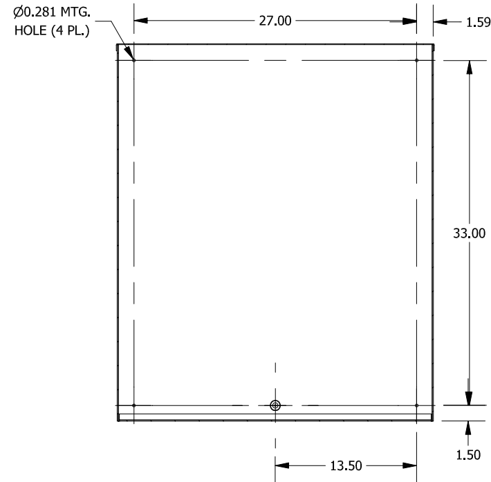
SECTION A-A (INSIDE BACK OF ENCL.)
