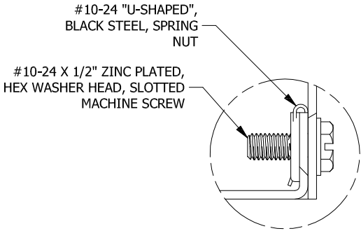
DETAIL A (4 PL.) (LID ATTACHMENT DETAIL)
